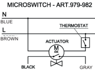
ELECTRIC CONNECTION FOR FOUR WIRE ACTUATORS WITH MICROSWITCH - ART.979-982
