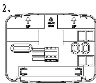
2. Fix the base on wall with provided screws
